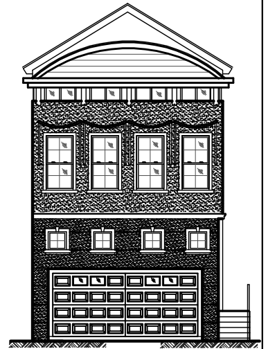
FRONT ELEVATION
